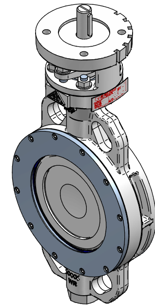
WAFER TYPE
