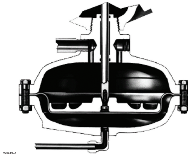
DETAIL OF TYPE 1098H ACTUATOR
