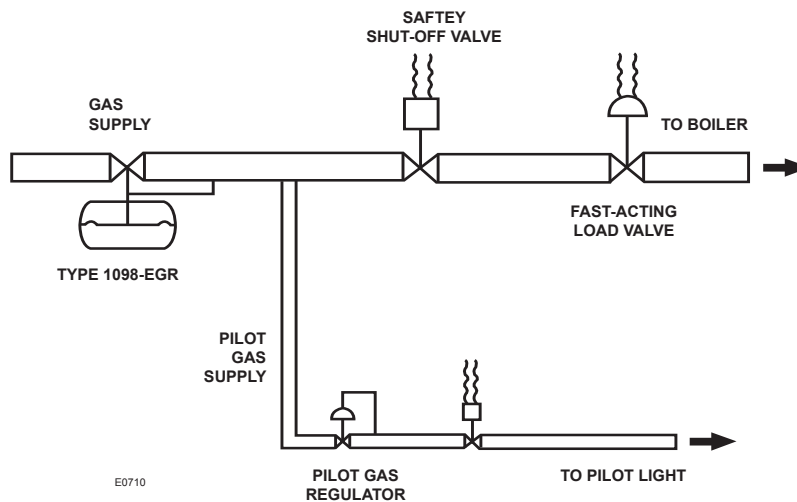
Figure 7. Boiler Fuel Configuration Installation Guide
