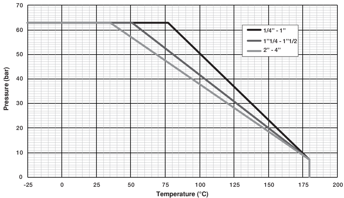
X3444 S - Pressure / Temperature diagram
